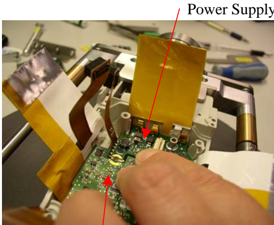
Figure 3. Radio and Power Supply Boards
