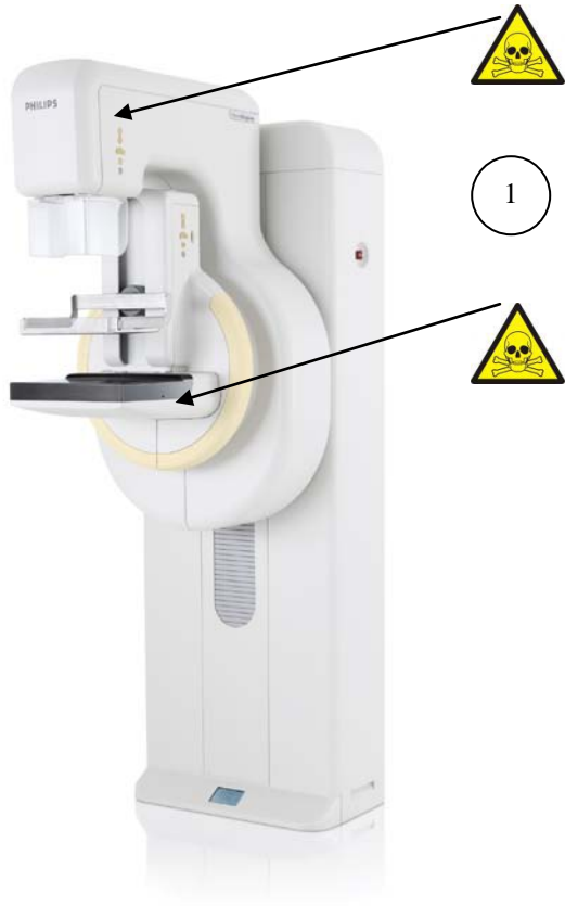
MammoDiagnost DR – Basic Unit (508 kg)
