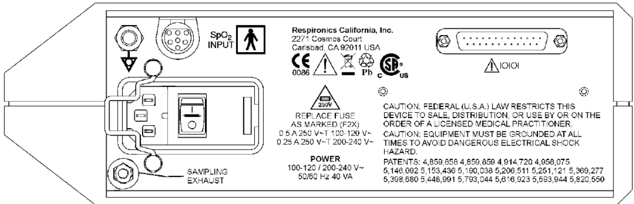
Rear View
