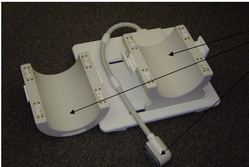
Figure 2 7T Invivo Quadrature Extremity coil – top and bottom separated.
