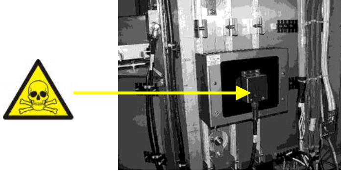
Figure 1, Cooling assembly with resistor (4522 132 3683X) containing beryllium-oxyde
