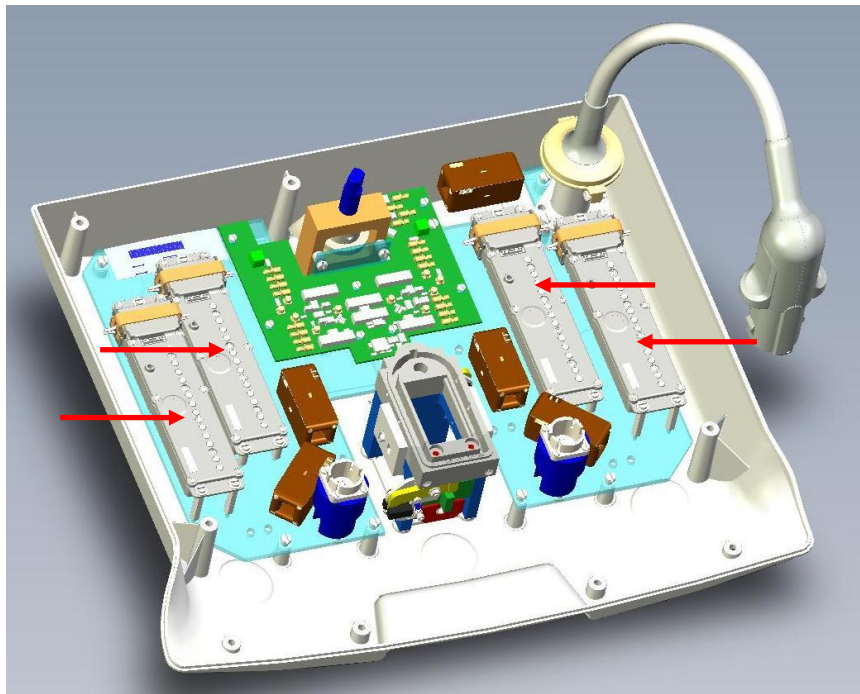
Figure 2, dStream Interface 1.5T RXE locations
