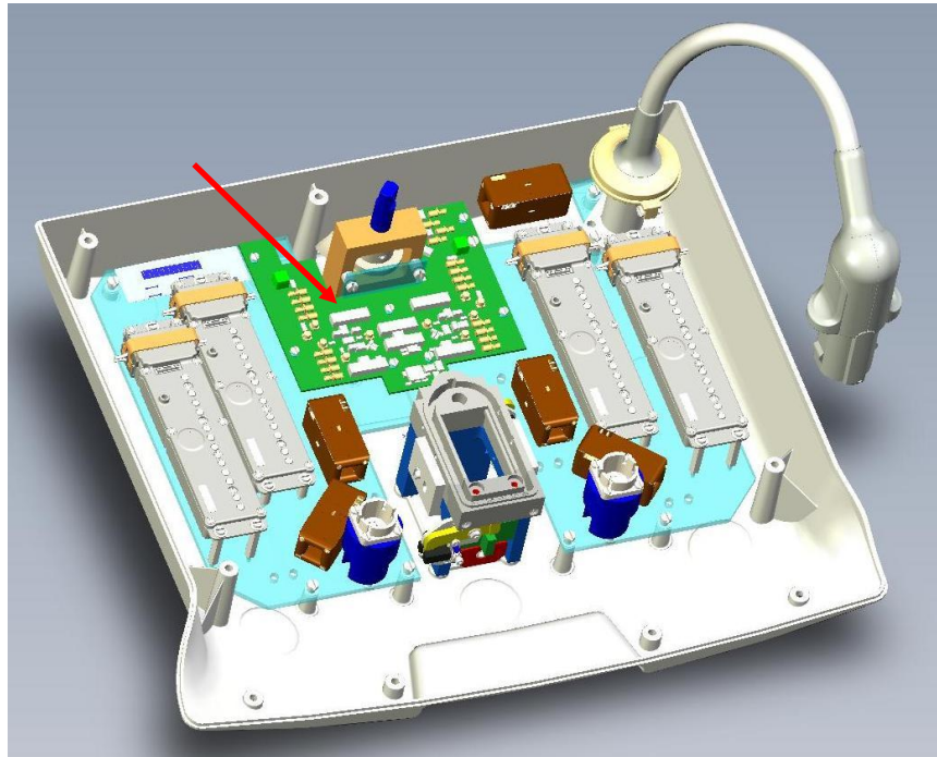
Figure 1, dStream Interface 1.5T pcb location
