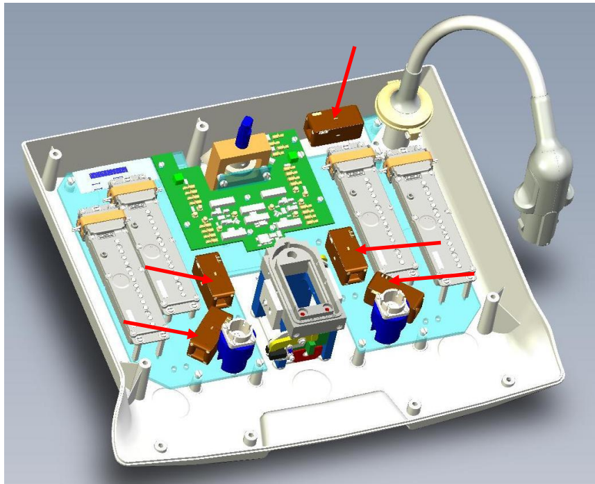
Figure 3, , dStream Interface 1.5T RF trap locations
