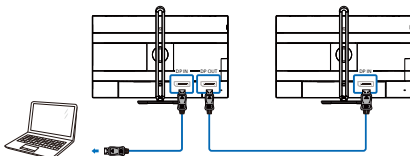
Multi-stream transport
