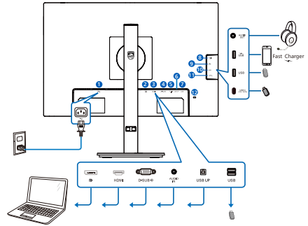
USB hub
