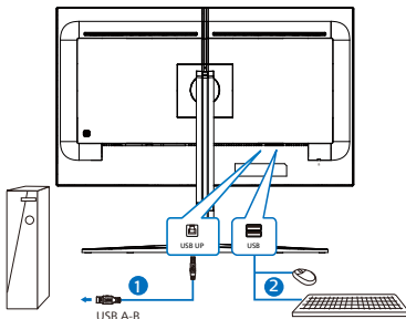
USB hub
