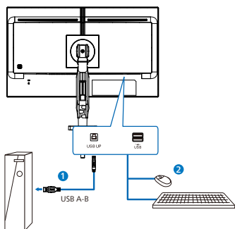
USB hub
