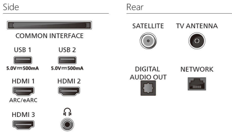
Connections 43PUS8000/50PUS8000/55PUS8000
