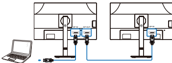
Multi-stream transport
