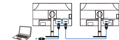
Multi-stream transport
