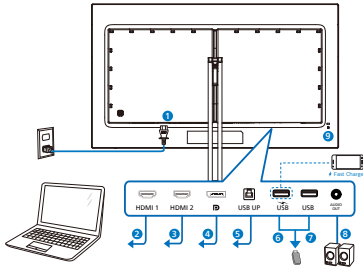
USB hub
