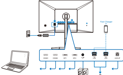
USB hub
