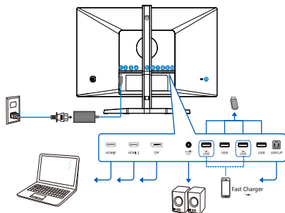
USB hub
