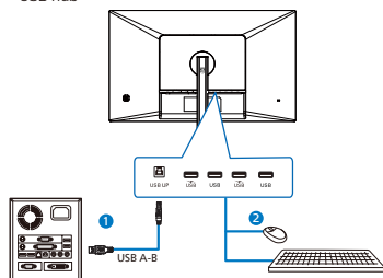
USB hub
