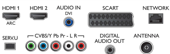
Rear
