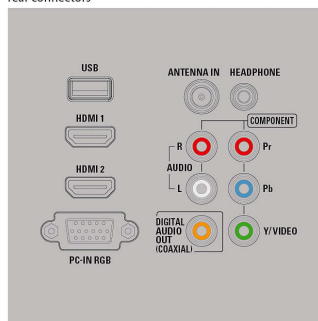
rear connectors
