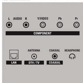
rear connectors
