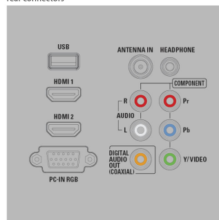
rear connectors
