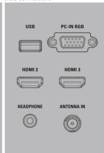
side connectors
