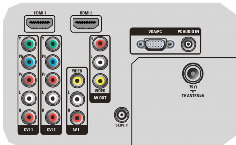
Rear connectors
