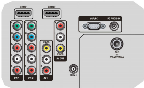
Rear connectors
