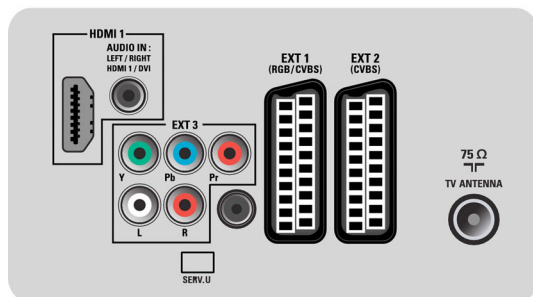
Rear connectors
