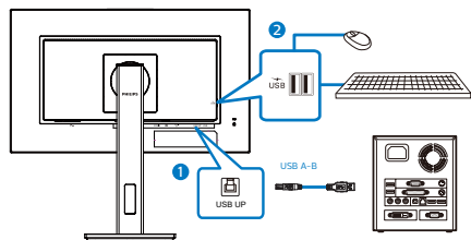
USB hub
