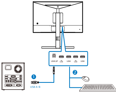
USB hub
