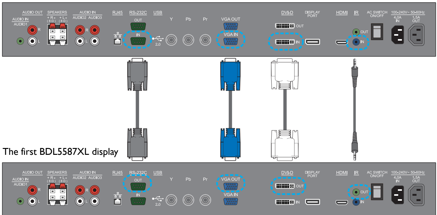
Additional BDL5587XL display
