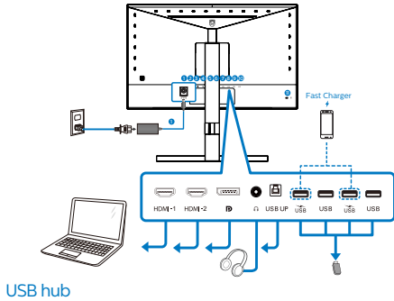
USB hub
