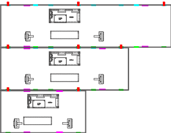
L-4-3-2 Installation
