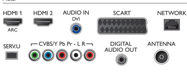
Rear
