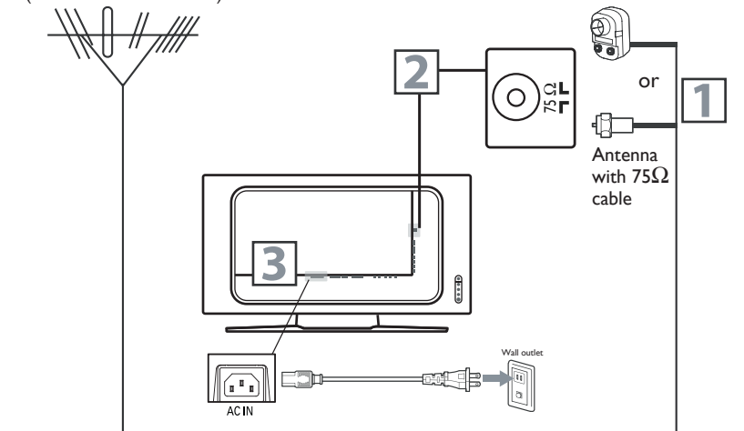
Outdoor or Indoor Antenna (Combination VHF/UHF)
