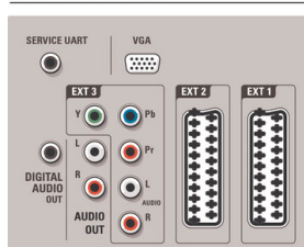
Rear connectors
