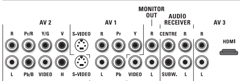
connectors
