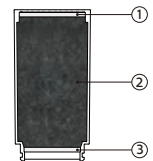
① PP棉 ② 颗粒活性炭 ③ PP棉
