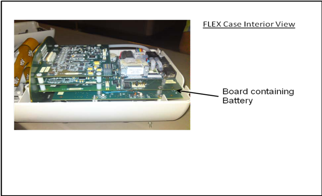
Figure 3 (Disassembly Instruction)
