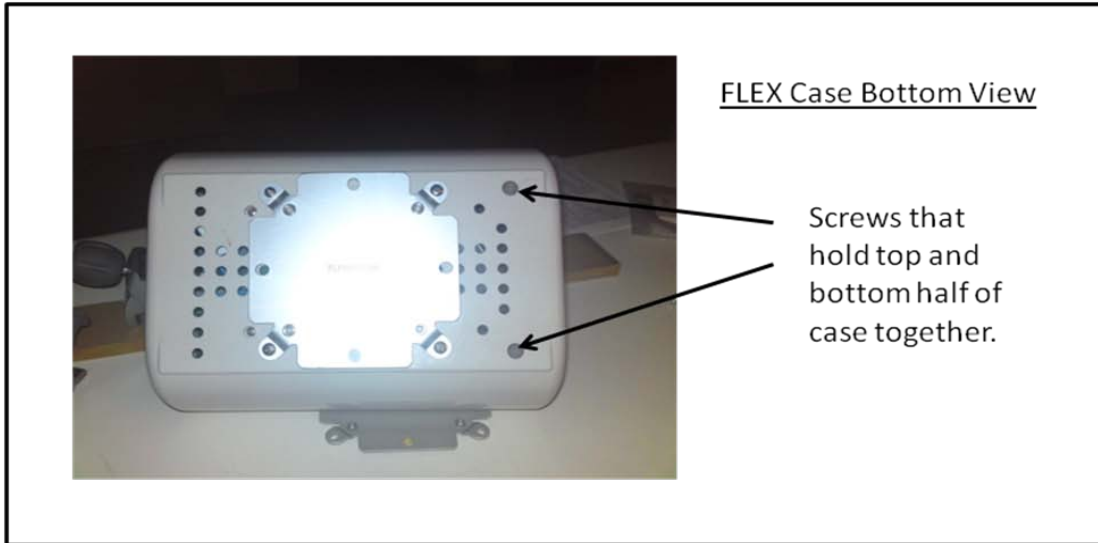
Figure 1 (Disassembly Instruction)
