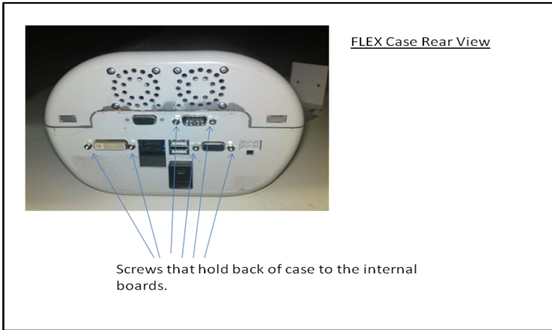
Figure 2 (Disassembly Instruction)
